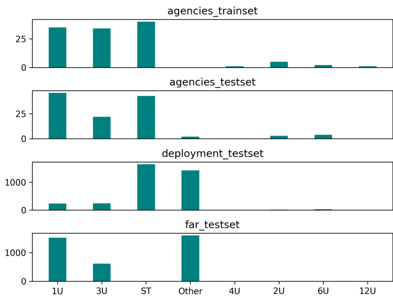
Figure 5. Number of Objects per Each Dataset
