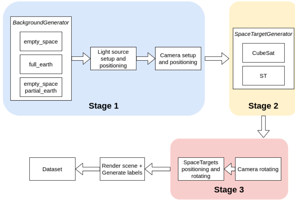
Figure 2. Blender Image Rendering Pipeline
